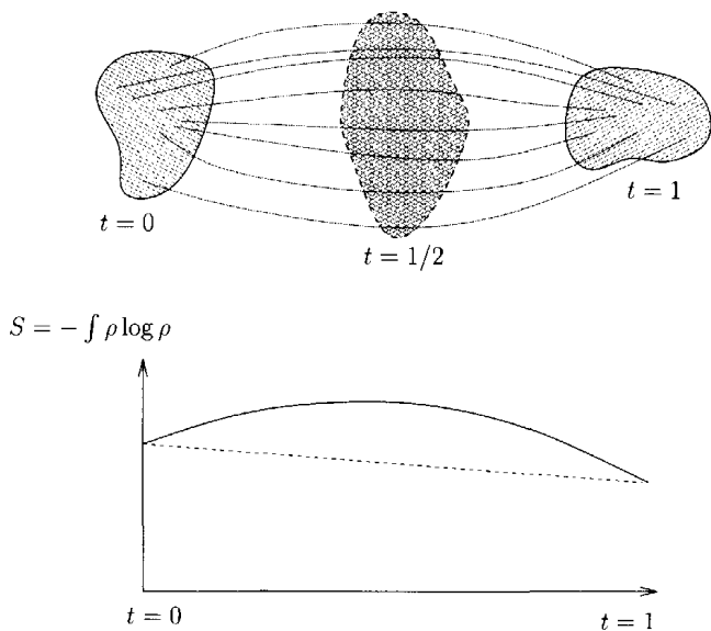
FIG. 7.2 – The lazy gas experiment: To go from state 0 to state 1, the lazy gas uses a path of least action. In a nonnegatively curved world, the trajectories of the particles first diverge, then converge, so that at intermediate times the gas can afford to have a lower density (higher entropy).
