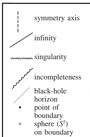
Fig. 2.37 Key for strict conformal diagrams.
