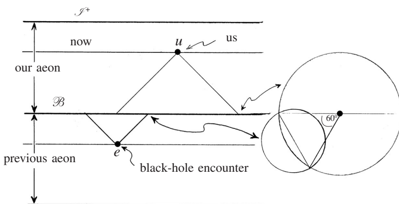
Fig. 3.28 We appear to be about \frac{2}{3} of the way up our aeon, in a conformal diagram. If this applies also to the earliest black-hole encounters in the previous aeon, then a cut-off in angular correlations at 60^\circ is to be expected.
