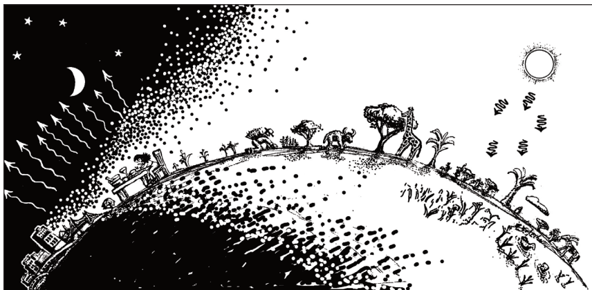
Fig. 2.9 Photons arriving at the Earth's surface from the Sun have higher energy (shorter wavelength) than those returned to space by the Earth. Given an overall energy balance (the Earth does not get hotter over time), there must be more photons leaving than arriving; that is, the energy arriving has lower entropy than that departing.
