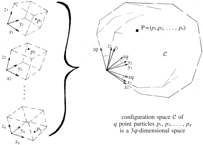
Fig. 1.4 Configuration space \mathcal{C} of q point particles p_1, p_2, \dots, p_q is a 3q -dimensional space.
