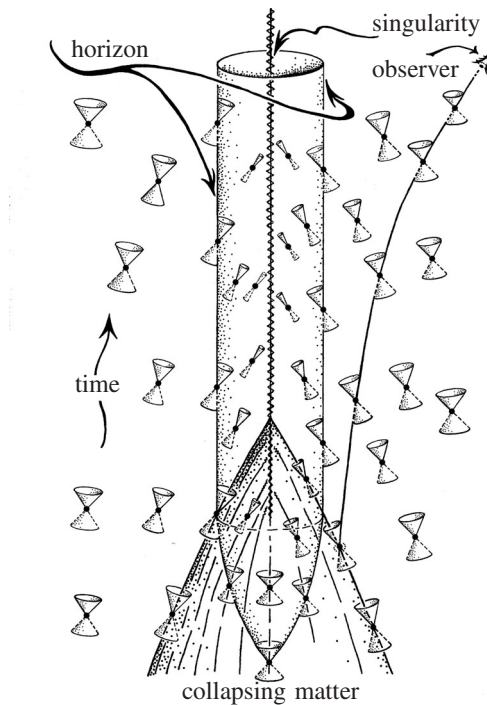
Fig. 2.24 Collapse of an over-massive star to a black hole. When the inward tilt of the future cone becomes vertical in the picture, light from the star can no longer escape its gravity. The envelope of these cones is the event horizon.
